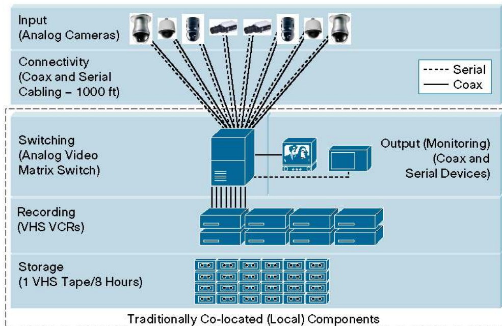
Figure 2 Analog Video Surveillance System
